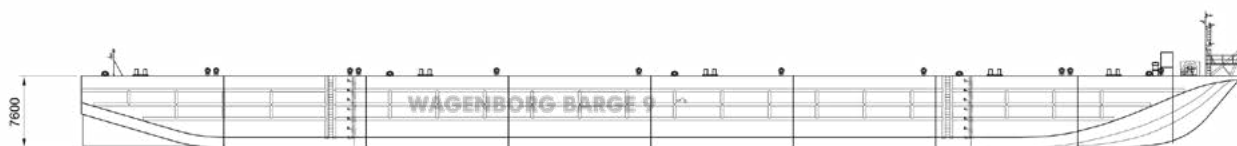
OUTBOARD PROFILE
